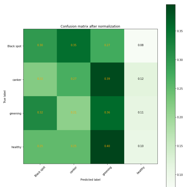
Figure 7: Inception V3 confusion matrix
